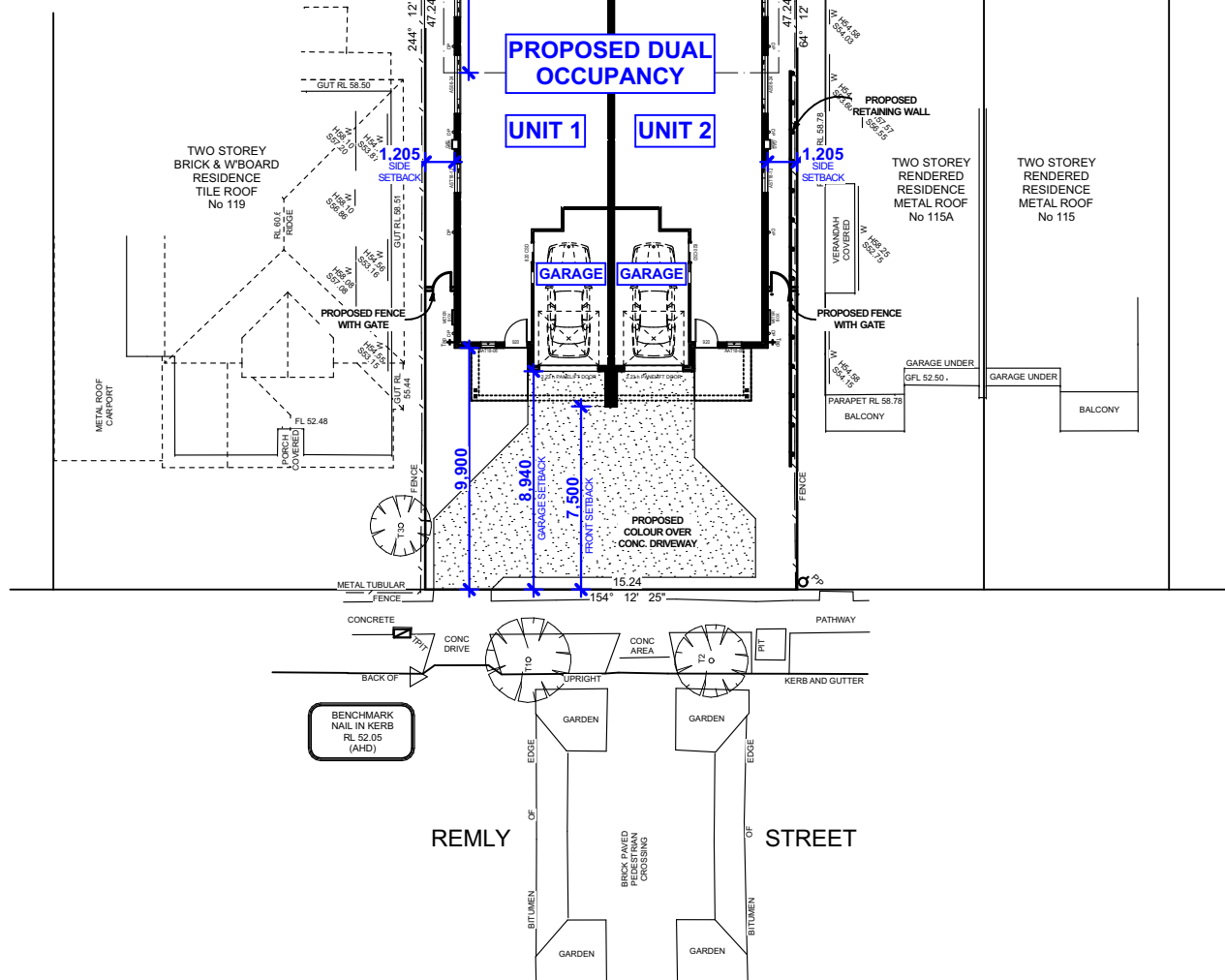
Proposed Site Plan Not To Scale
